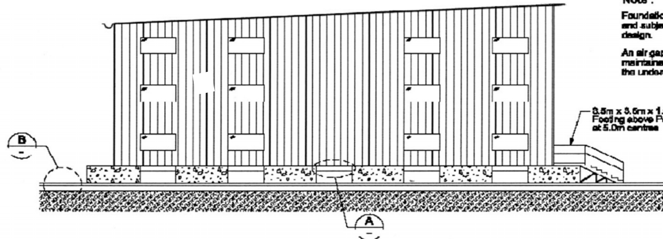
Figure 8: Mitigation Design at Works Area B 圖 8: 乙施工區的緩解設計
