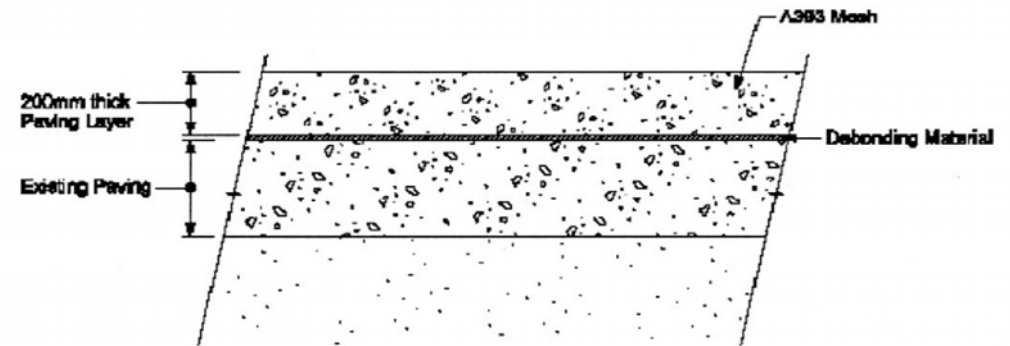
Detail B 1:30
